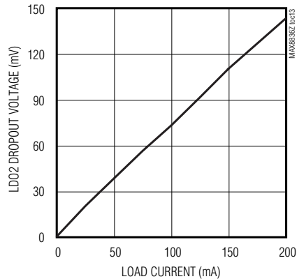
LD02 DROPOUT VOLTAGE vs. LOAD CURRENT
